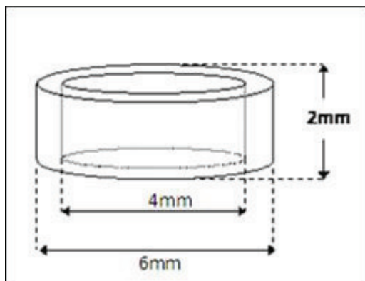
Figure X — (6) — Cylindrical gauge for measurement of projectile tips
