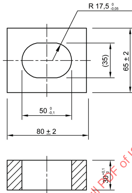
Figure 23 — Test template A
