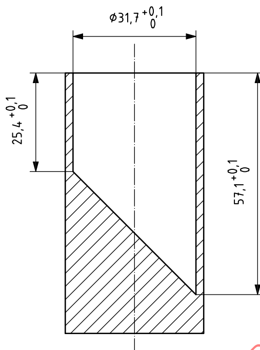
Figure 22 — Small parts cylinder
