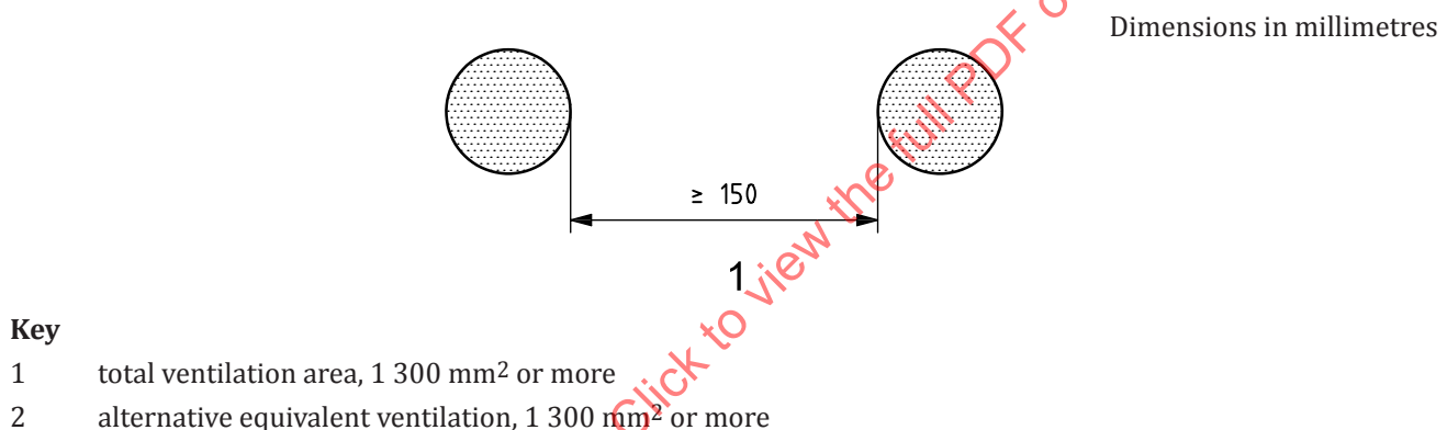
Figure 17 — Example of an equivalent single ventilation opening
