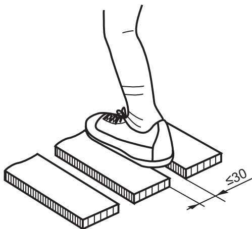
Figure 10 — Measurement of surface gap on running and walking levels
