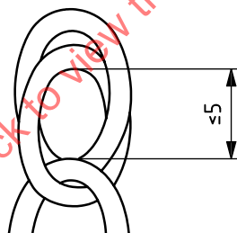
Figure 15 — Maximum openings in chains for swings
