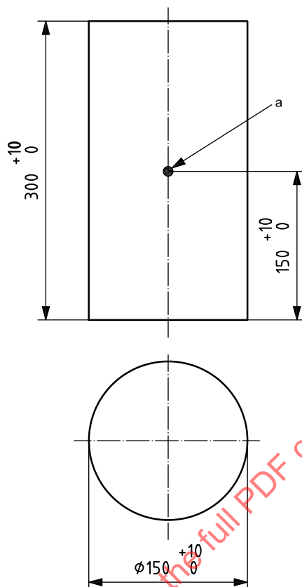
Figure 16 — Load for determination of strength and stability
