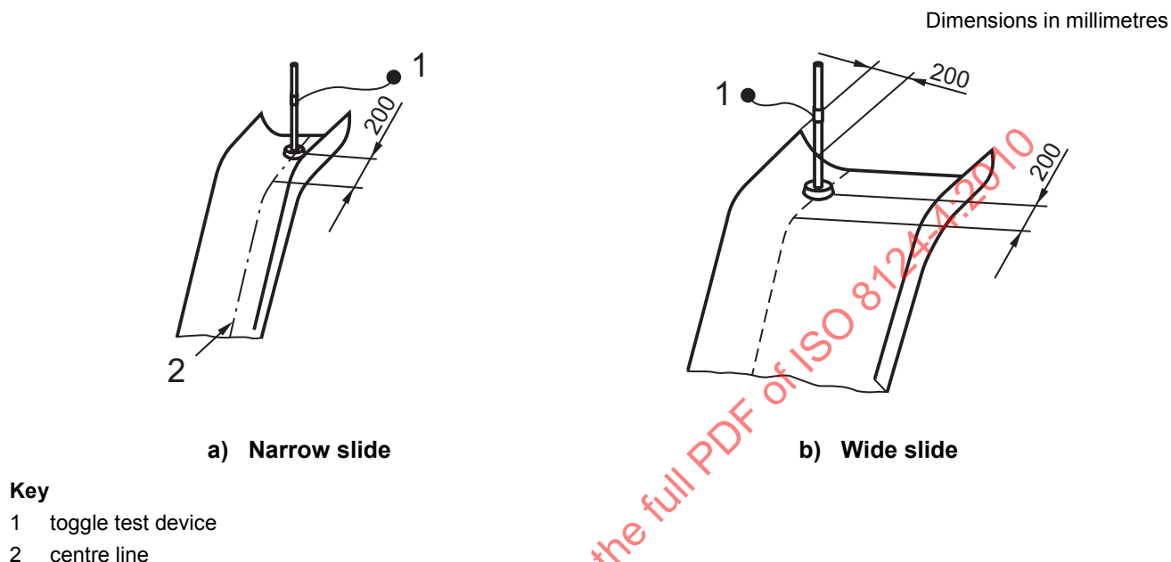
Figure 29 — Positioning of the test device on slides
