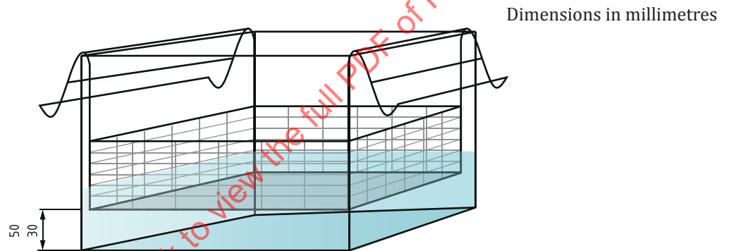
Figure E.2 — Water-filled ultrasonic bath with aluminium foil covering the basket
