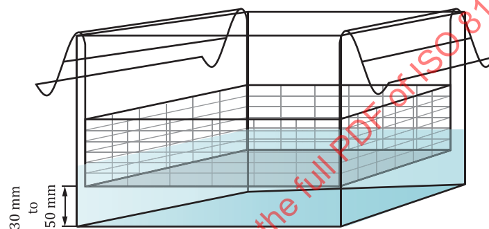
Figure E.2 — Water-filled ultrasonic bath with aluminium foil covering the basket
