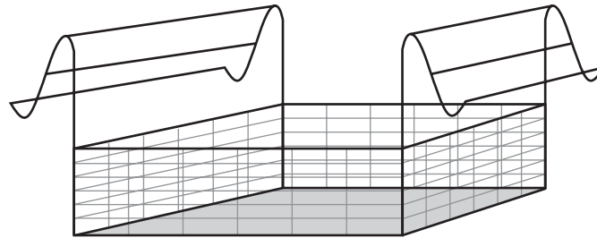
Figure E.1 — Basket covered with aluminium foil
