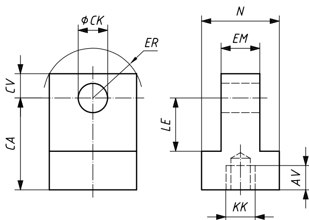
Figure 6 — AP4 — Rod eye plain, female thread
