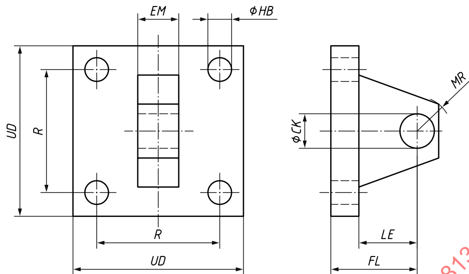
Figure 7 — AB2 — Eye bracket
