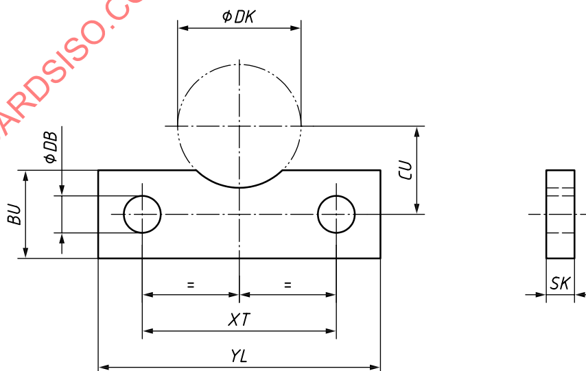
Figure 4 — AL6 — Locking plate for pivot pin
