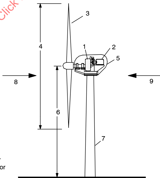
Figure A.1 - Horizontal axis wind turbine (HAWT)
