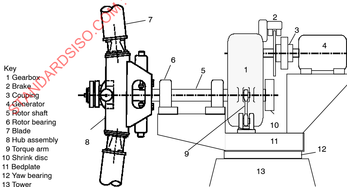
Figure A.2 - Schematic of nacelle layout for a HAWT
