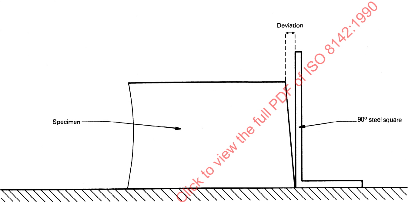
Figure B.1 — Measurement of deviation from squareness
