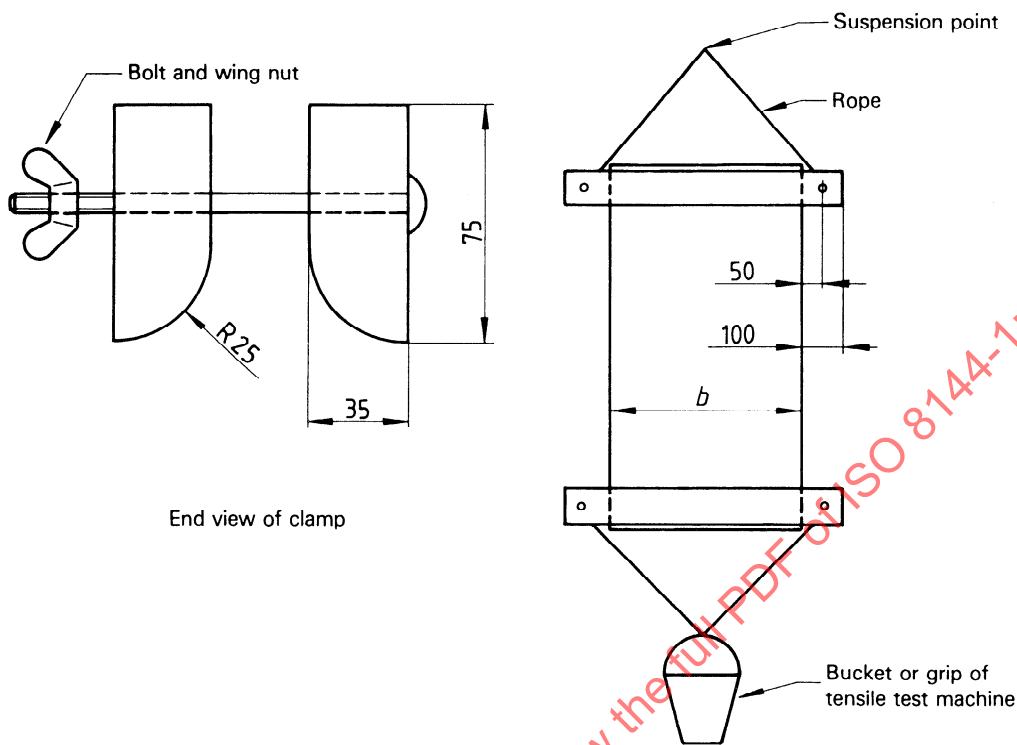
Figure B.1 — Suspended assembly
