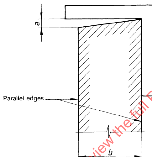
Figure A.5 — Measurement of squareness
