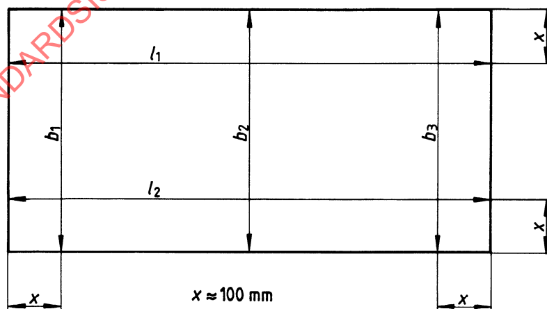
Figure A.1 — Location of measurements for length and width
