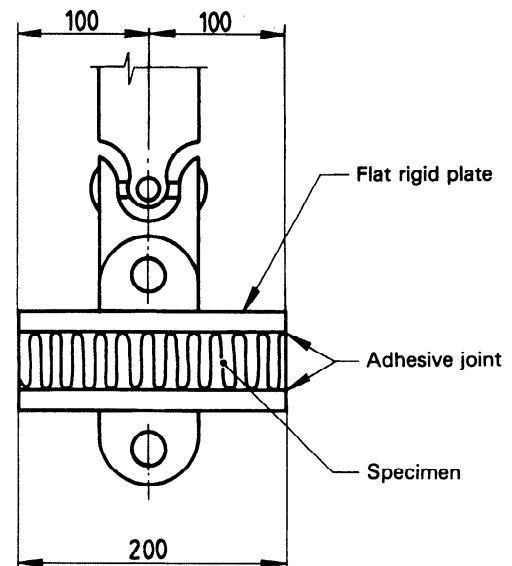
Figure C.1 — Interlaminar strength test
