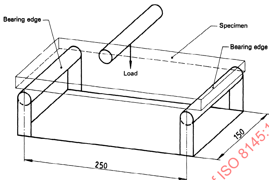
Figure D.1 — Breaking load test apparatus
