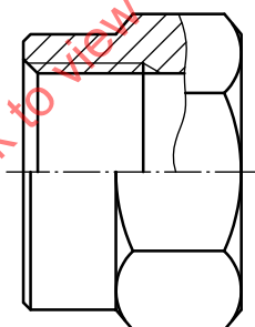
Figure 15 — B-nut
