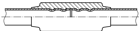
Figure 13 — Shape-memory-alloy permanent fitting
