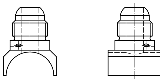
Figure 28 — Semi-casing fitting
