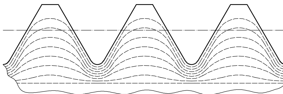
Figure 3 — Grain flow in threads (see 5.5.2)
