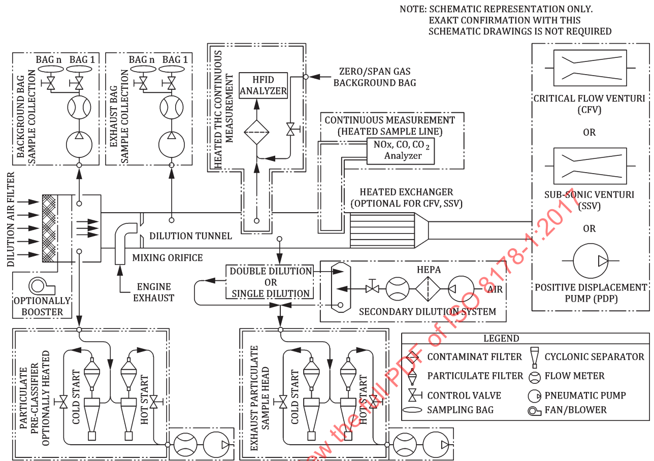
Figure 9 — Full-flow dilution system
