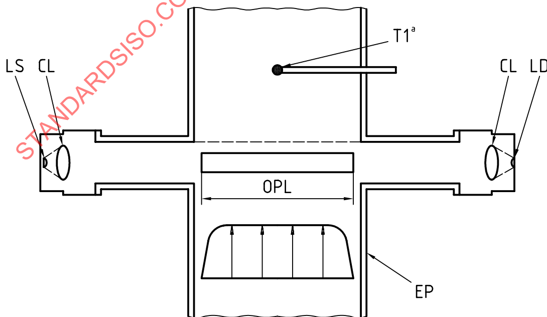
Figure 1 — Full-flow opacimeter
