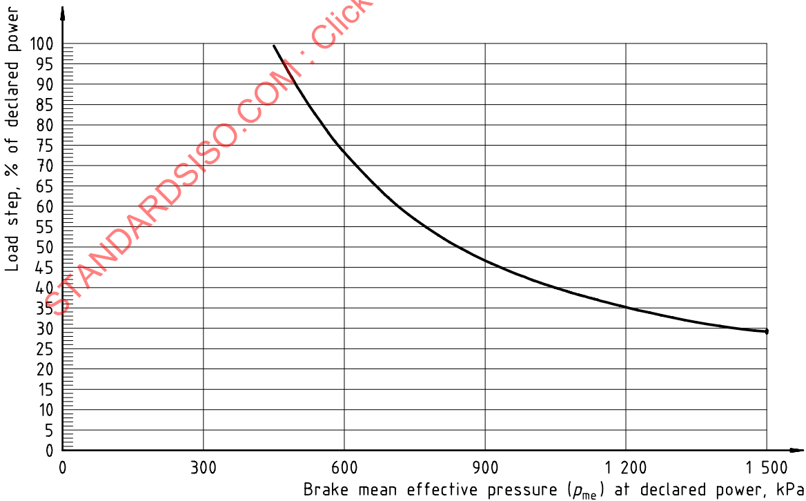
Figure B.2 — Load step for two-stroke engines
