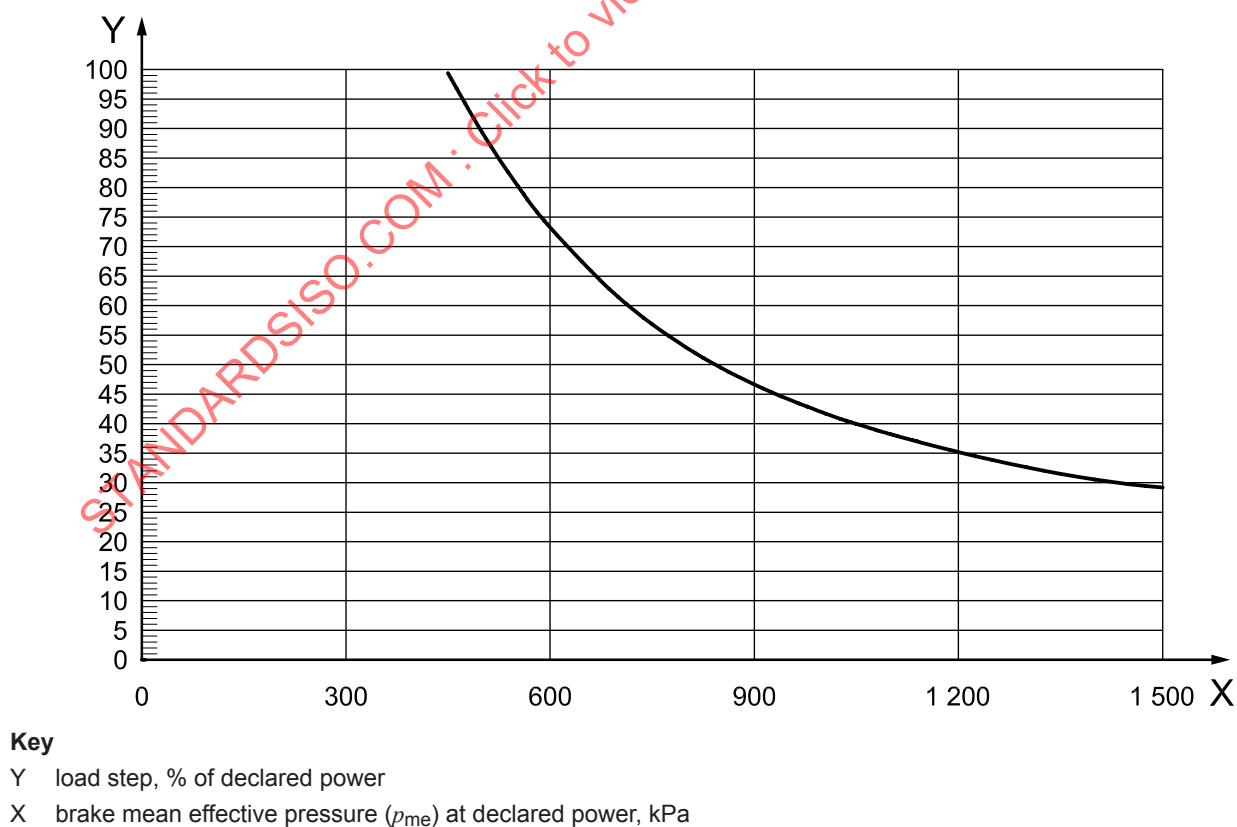
Figure B.2 — Load step for two-stroke engines
