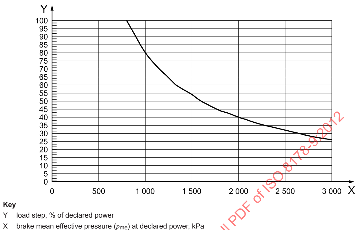
Figure B.1 — Load step for four-stroke engines
