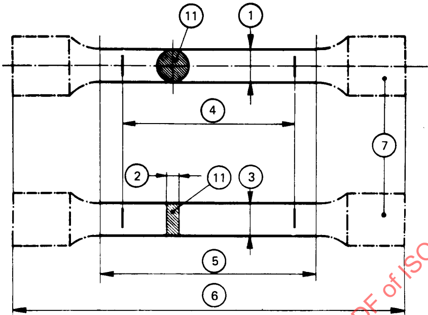
FIGURE 1 — Test pieces of circular and rectangular cross-section
