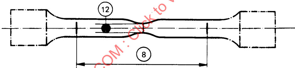
FIGURE 2 — Test piece of circular cross-section after fracture
