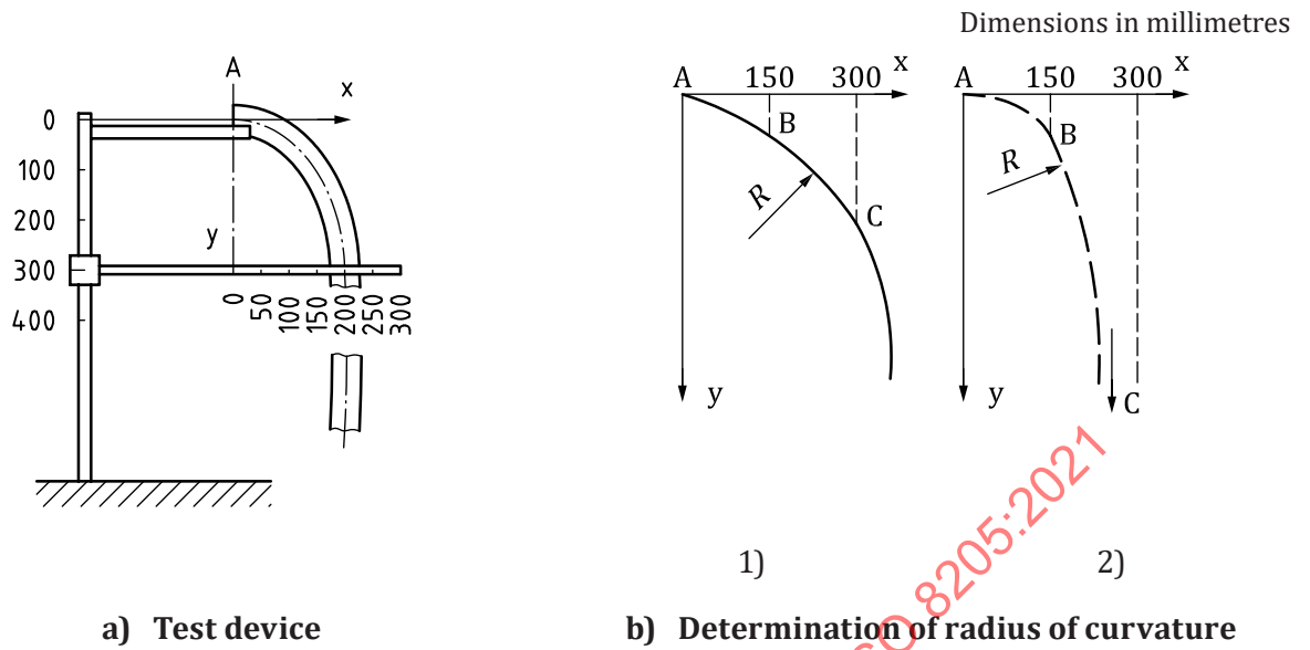
Figure 5 — Measurement of radius of curvature
