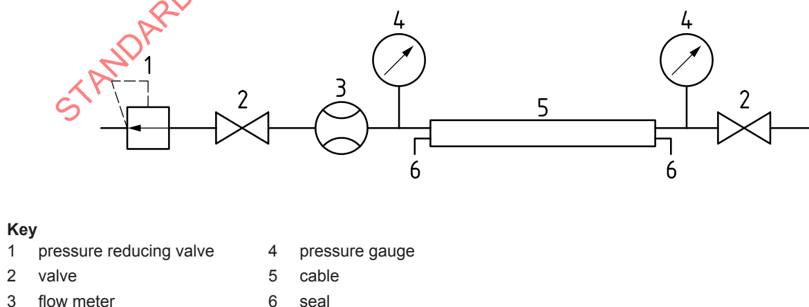
Figure 1 — Example of water supply to the cable
