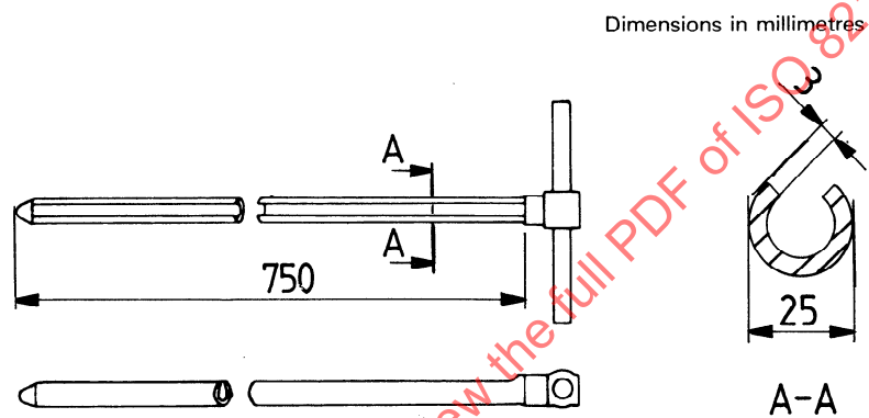
Figure 3 — Closed-end sampling spear
