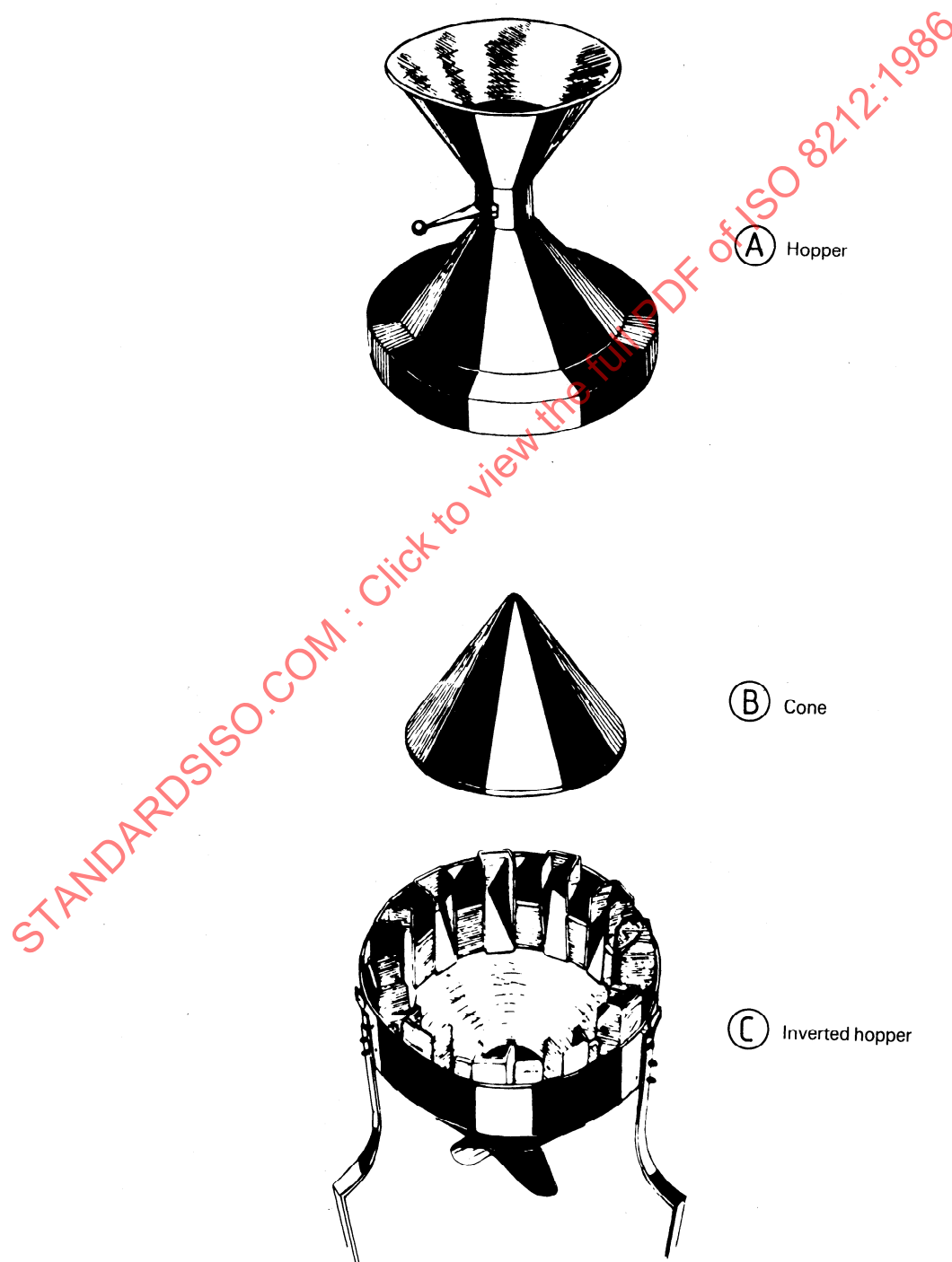
Figure 1a — Exploded view of a typical conical divider (see ISO 607)
