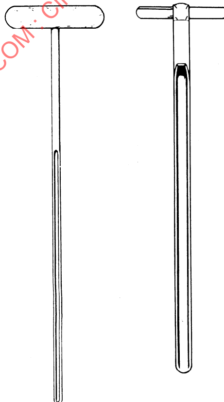
Figure 4 — Further designs of open-end sampling spears
