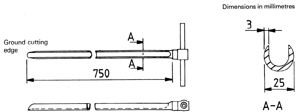
Figure 2 — Open-end sampling spear
