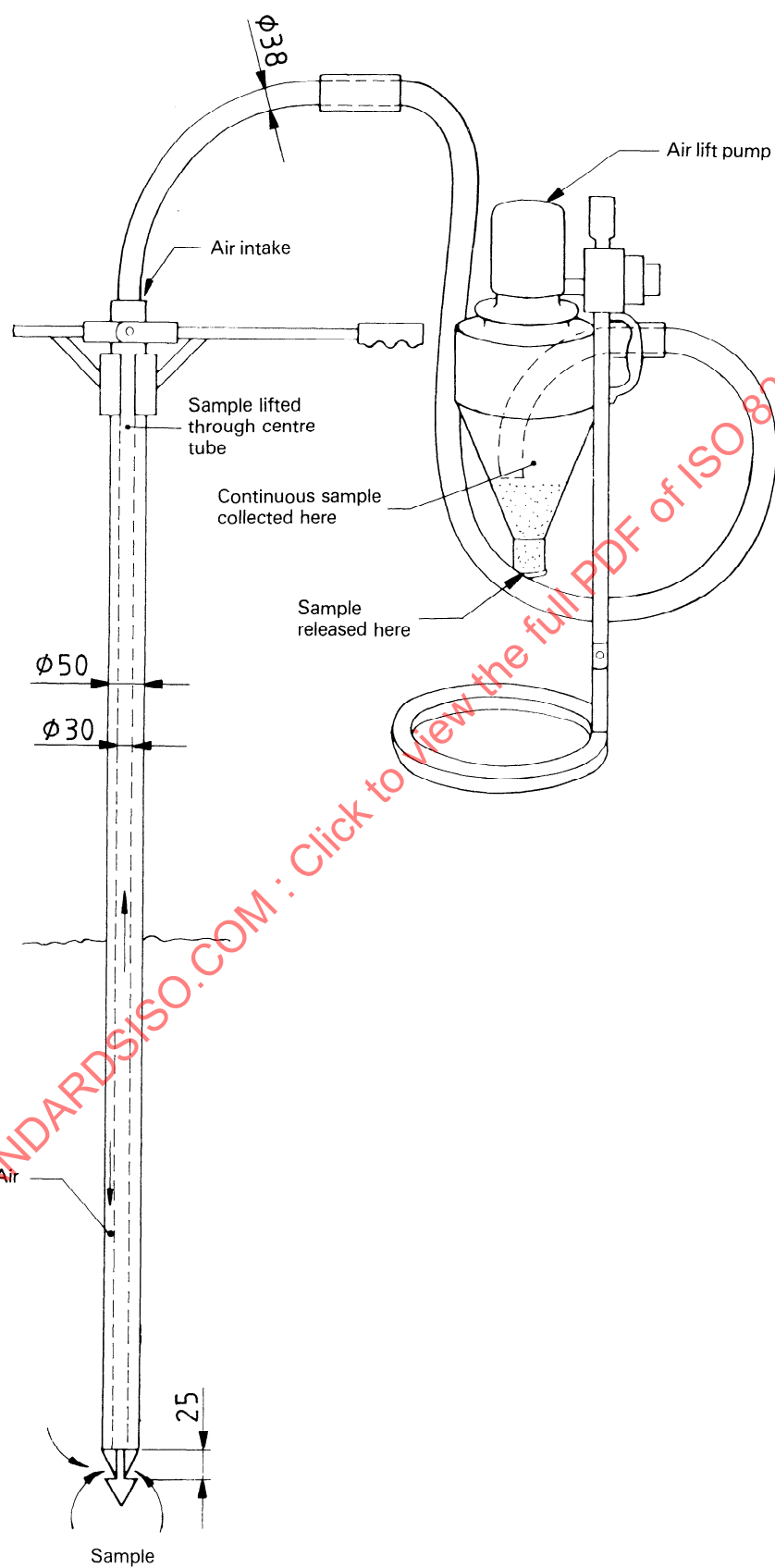
Figure 10 — Pneumatic probe sampler (see 4.1.2)
