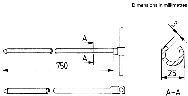
Figure 3 — Closed-end sampling spear
