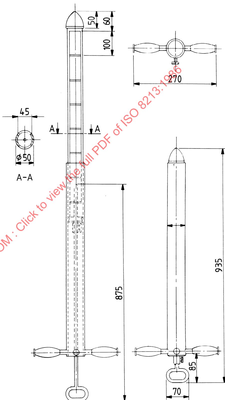
Figure 5 — Closable sampling spear
