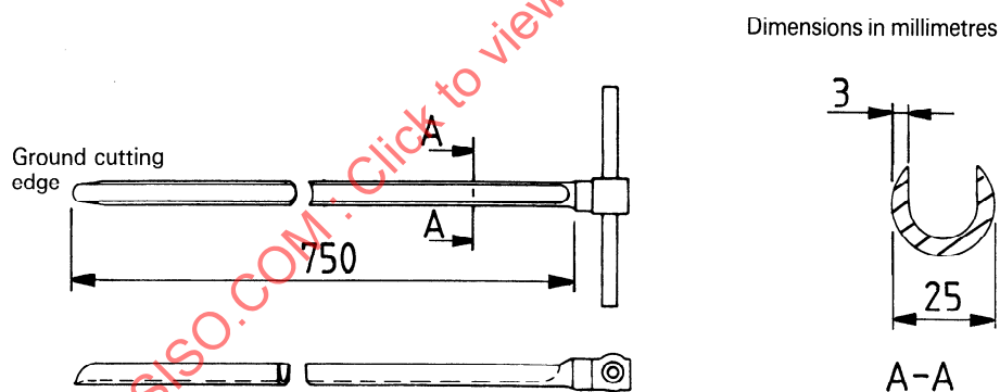
Figure 2 — Open-end sampling spear
