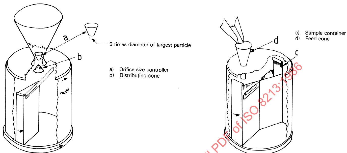
Figure 17 — Rotary sample dividers (see 4.1.3)
