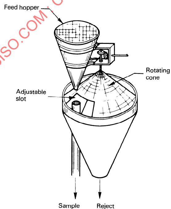
Figure 18 — Double-cone sample divider (see 4.1.3)
