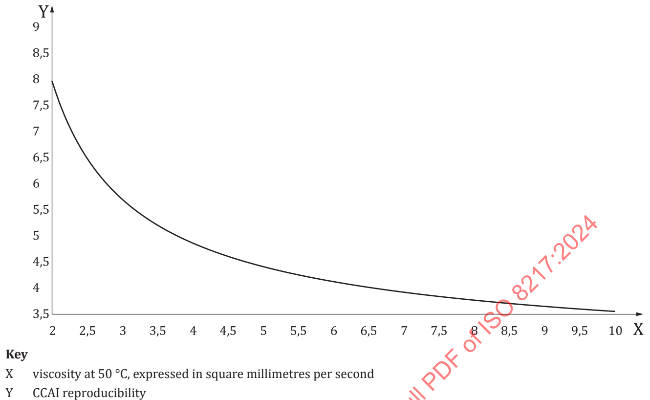
Figure C.2 — Plot of CCAI reproducibility against viscosity, 2 mm 2 /s to 10 mm 2 /s
