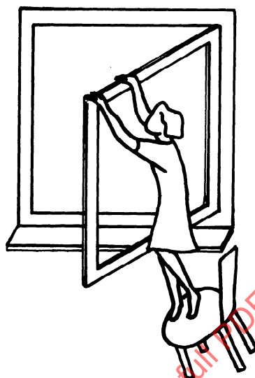
Figure 3 — Racking test situation with additional vertical force applied to window
