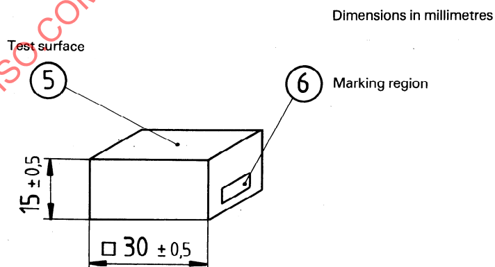
Figure 7 — Marking of each ferrite secondary standards
