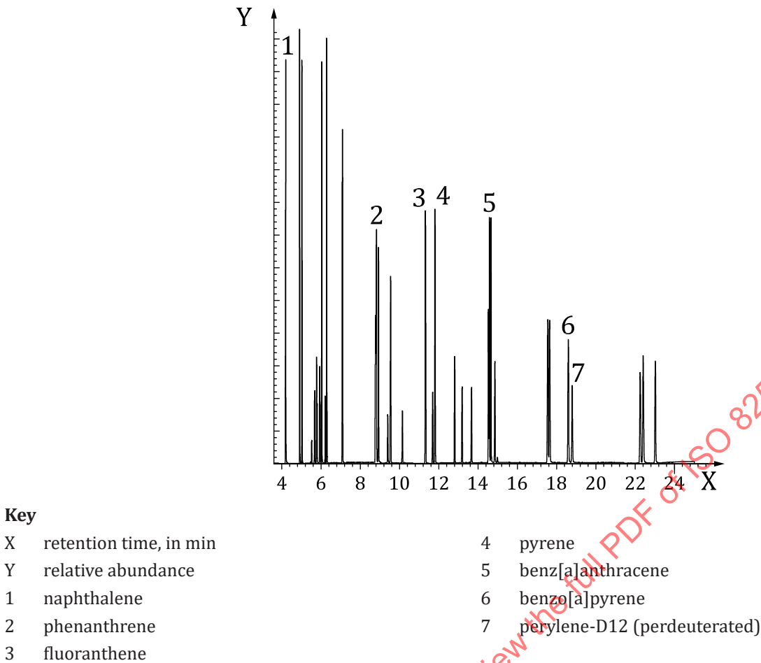
Figure D.2 — Chromatogram of a standard solution
