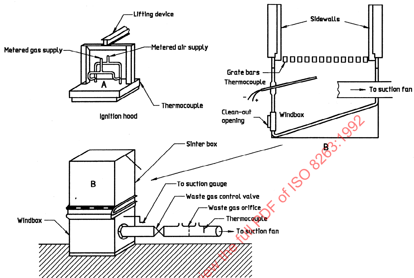
Figure 1 — Example of sintering test equipment
