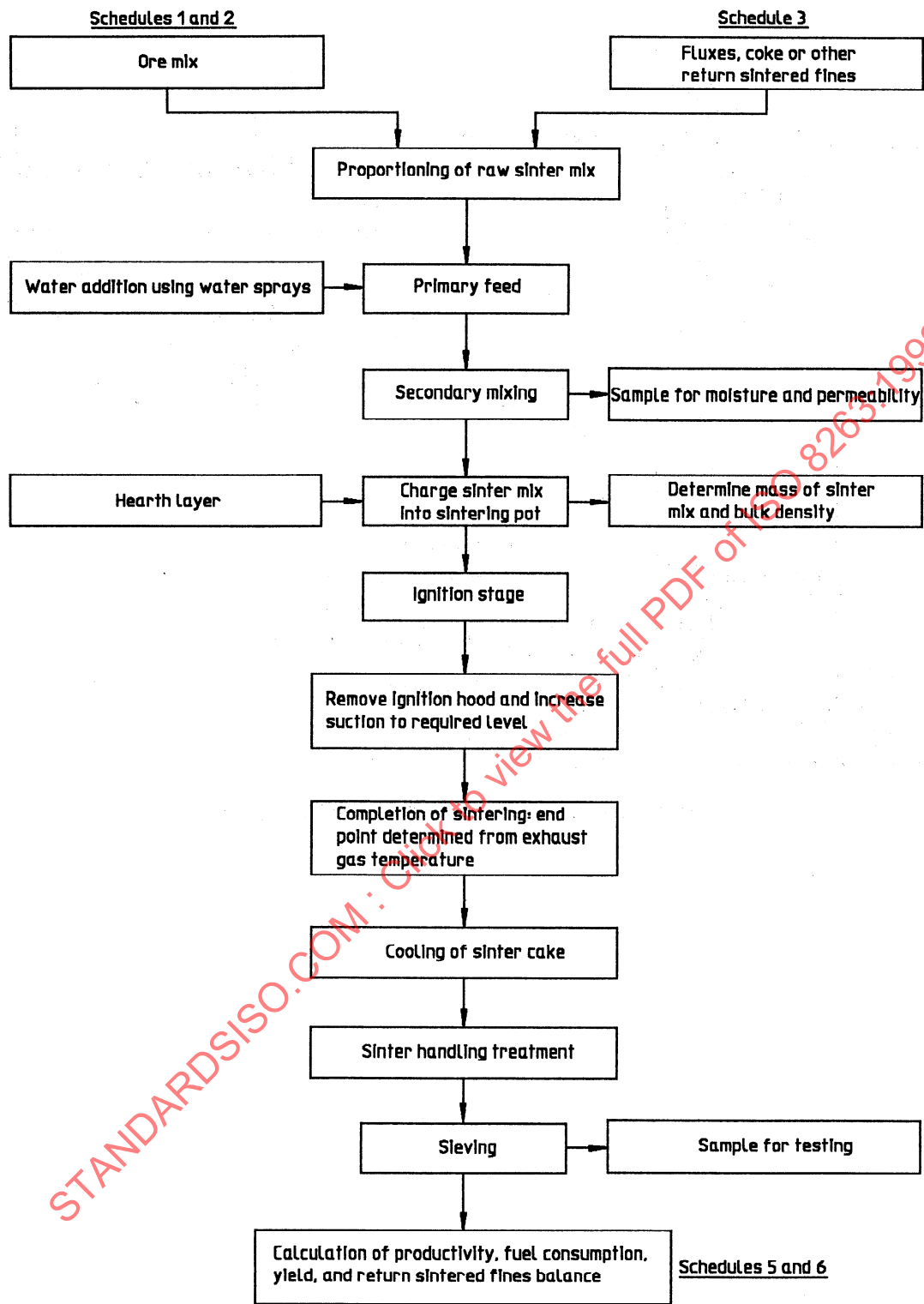
Figure 2 — Flowsheet of typical sinter test procedure
