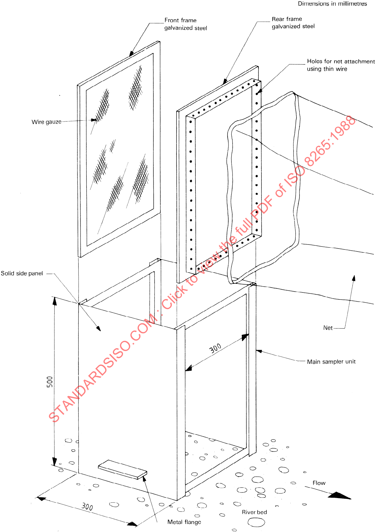
Figure 2 — Modified Surber sampler
