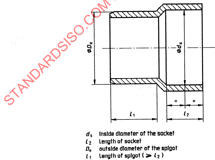
Figure 3 — Location of points of measurement for solvent cement sockets and spigots
