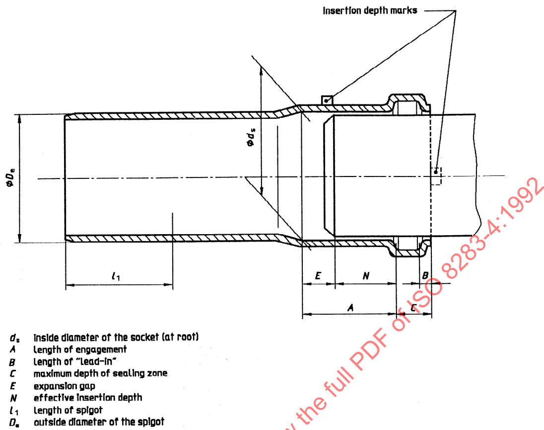
Figure 2 — Location of points of measurement for type L sockets and spigots
