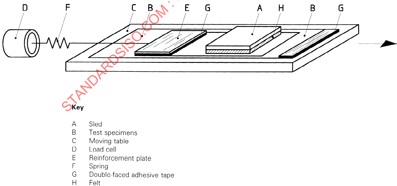
Figure 1 — Example of moving-table apparatus for determination of coefficients of friction
