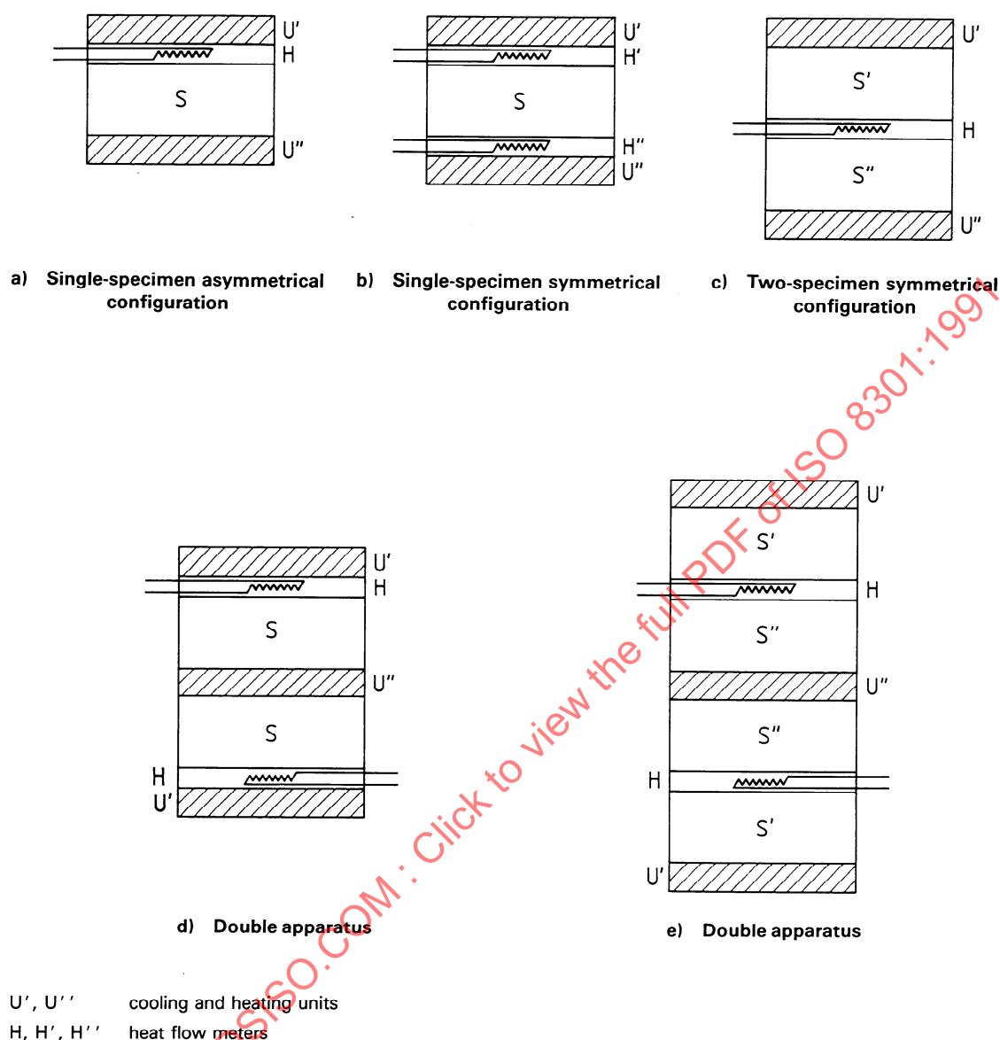
Figure 1 — Typical layouts of heat flow meter apparatus configurations
