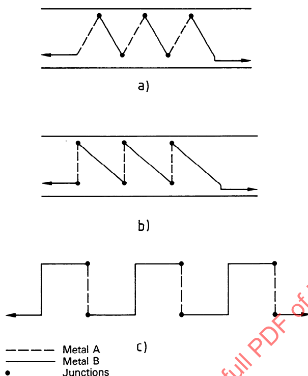
Figure 3 — Examples of schematic designs of thermopiles
