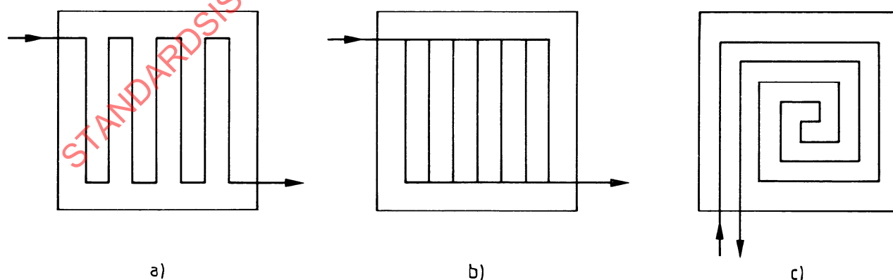
Figure 2 — Examples of schematic designs of heating and cooling units in the case of external liquid supply
