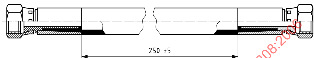
Figure 2 — Internal free length, with tolerance, of test piece
