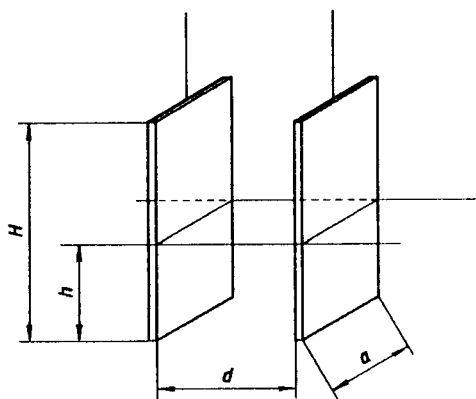
Figure A.1 — Basic diagram
