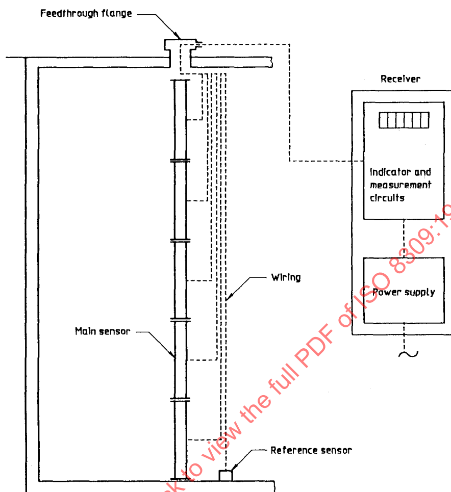
Figure 1 — Example of capacitance-type level gauge
