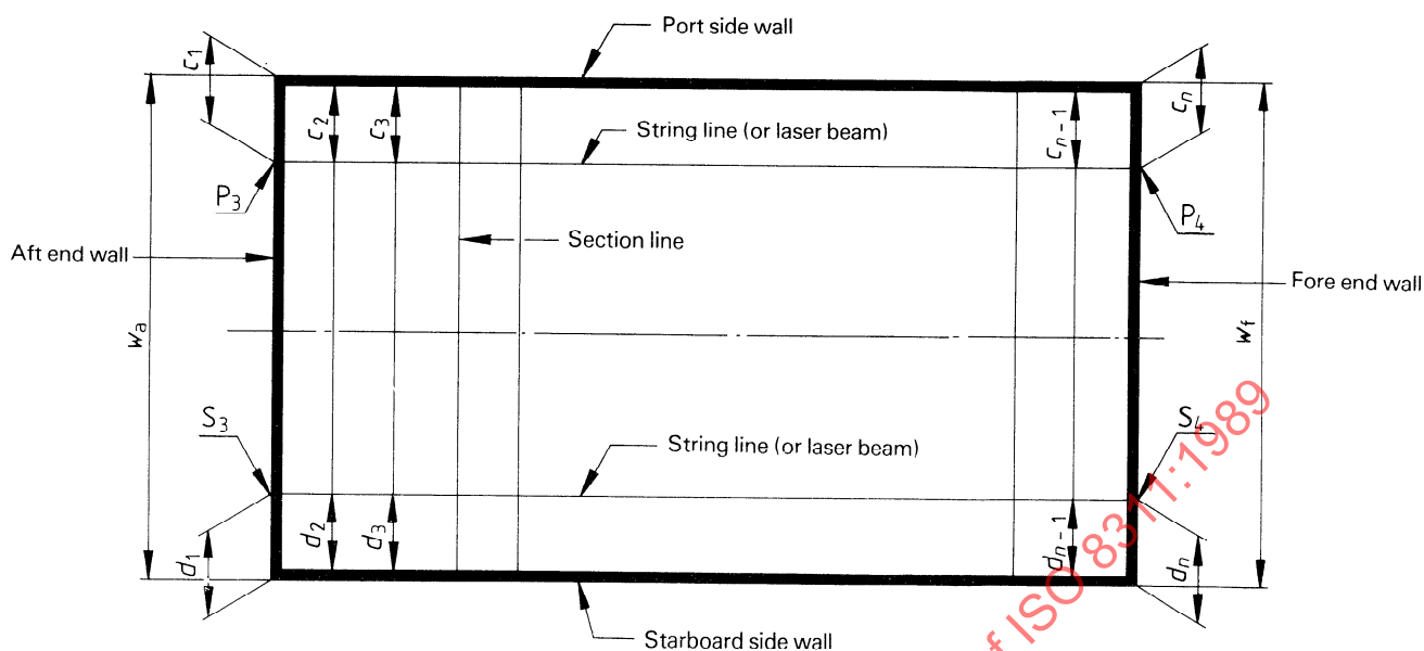
Figure 2 — Plan view of an intermediate horizontal plane
