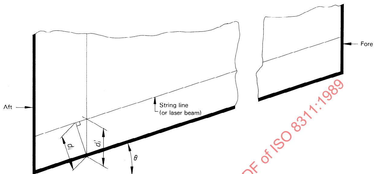
Figure 4 — Correction of offsets
