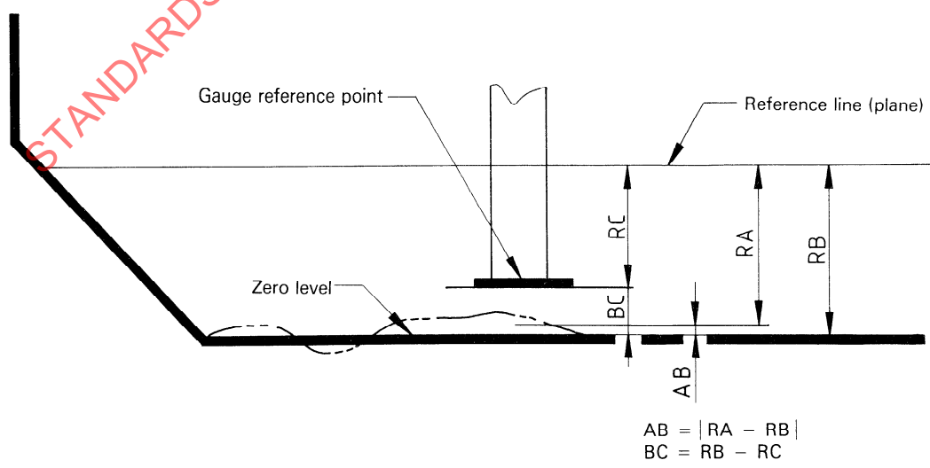
Figure 7 — Transverse section view of tank bottom
