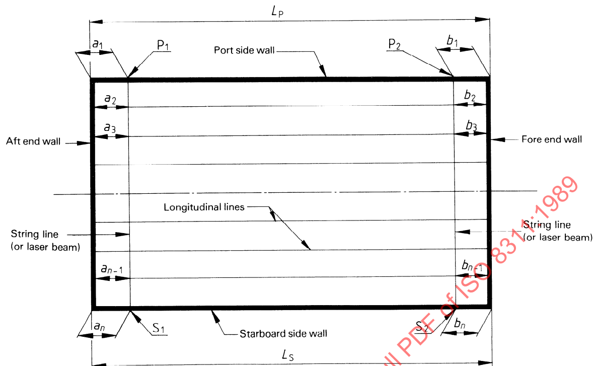
Figure 1 — Plan view of an intermediate horizontal plane
