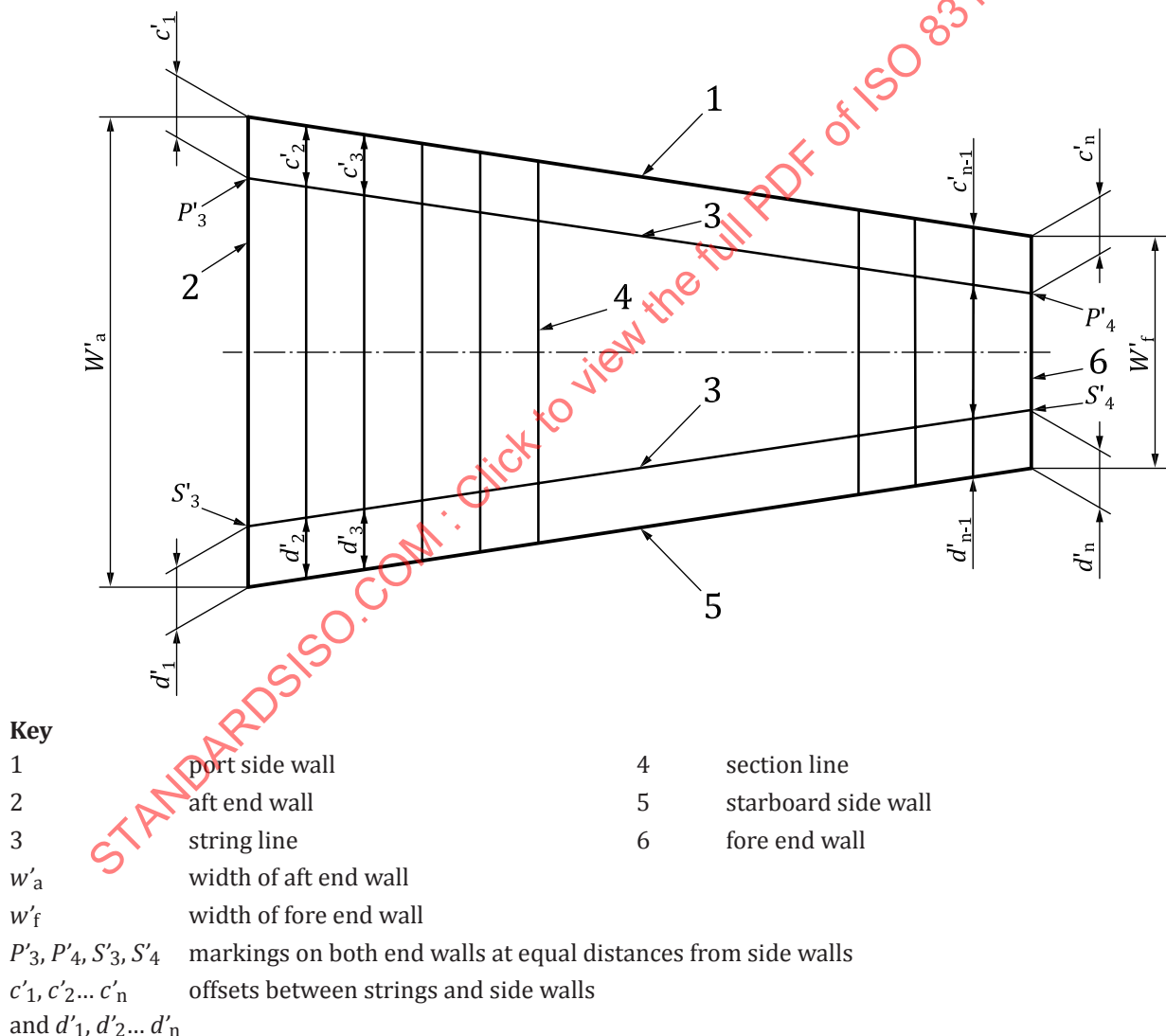
Figure 3 — Plan view of an intermediate horizontal plane (trapezoidal tank)
