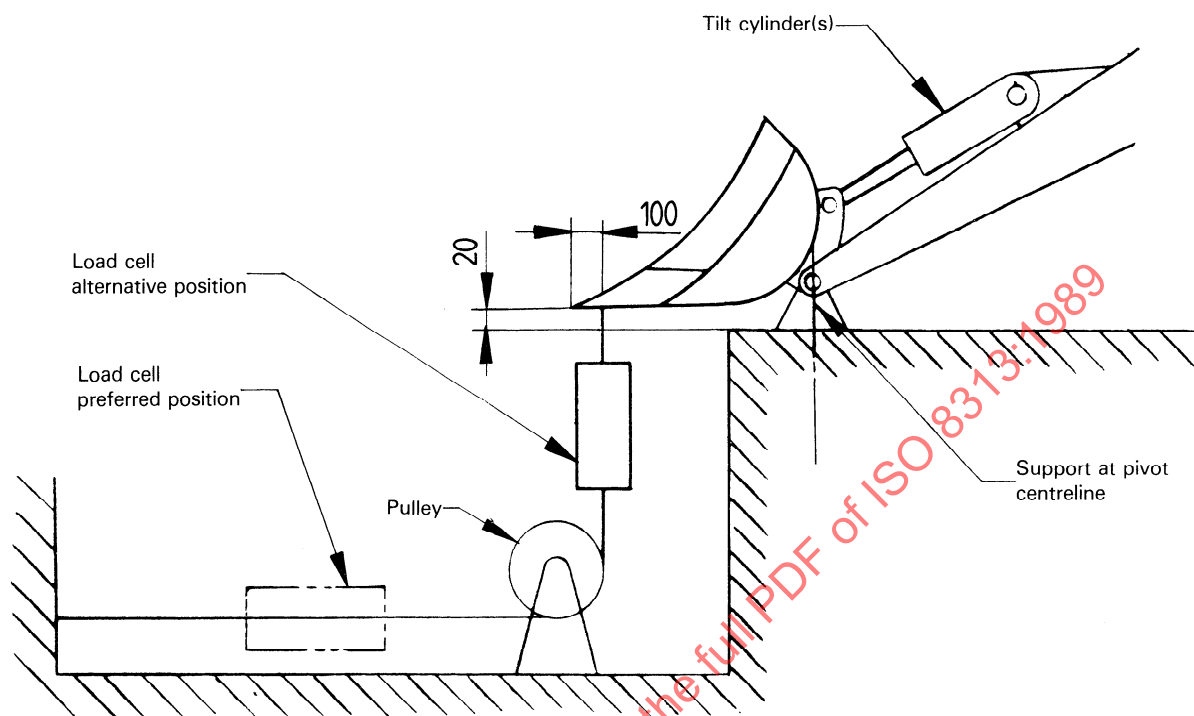
Figure 3 — Typical test arrangement for determination of maximum breakout force exerted by tilt cylinder(s)
