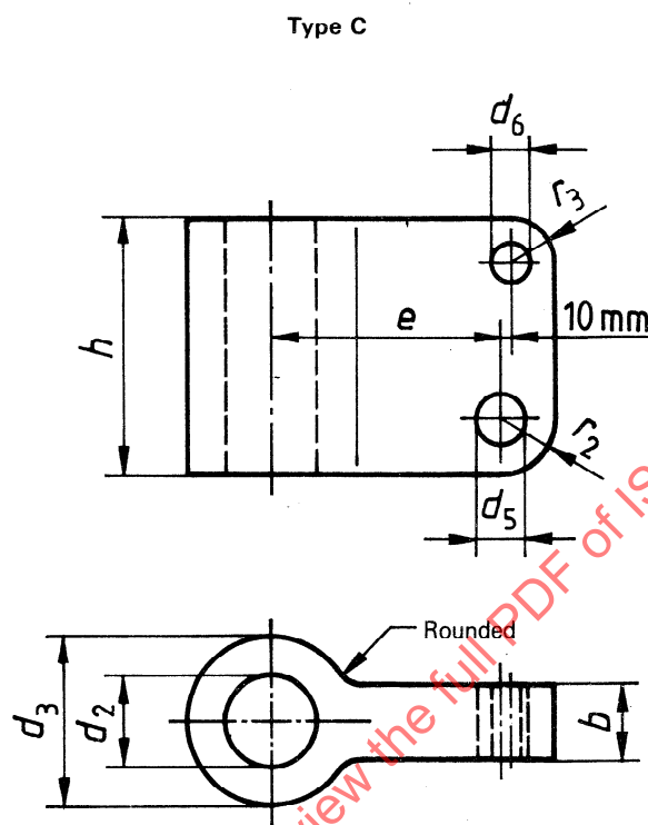
Figure 2 — Shape of trunnion piece, type C
