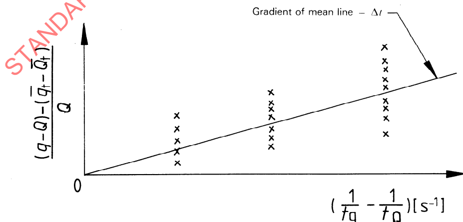
Figure 7 — Graph with plotting of results of diverter timer actuator tests, as given in A.1.2
