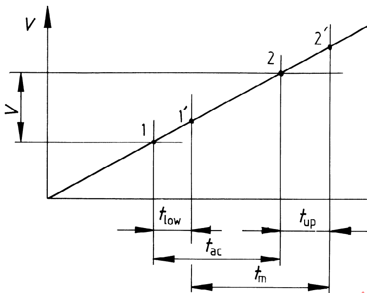
Figure 10 — Graph of volume collected against time at constant flow-rate
