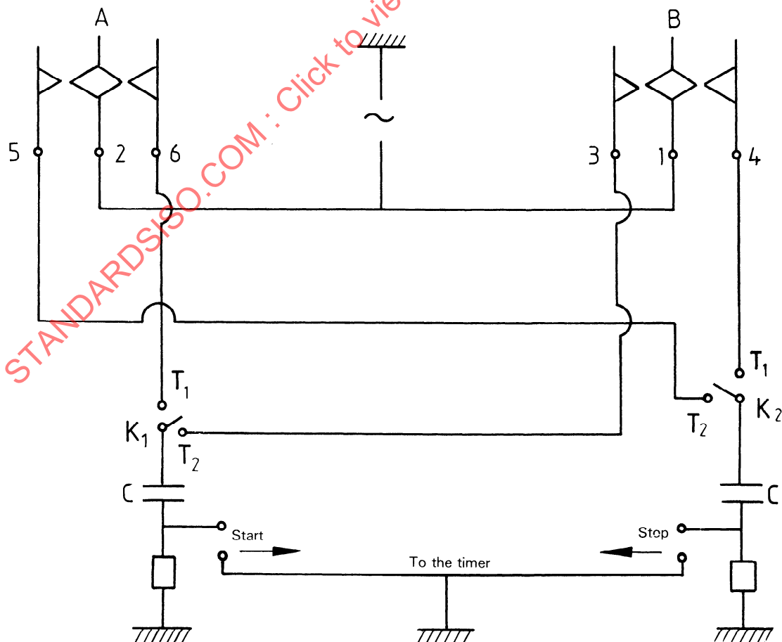
Figure 9 — Diagram of system for measuring the switching time and switching time difference of the diverter
