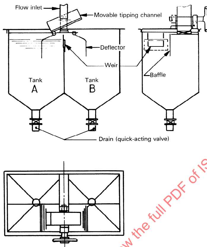
Figure 5 — Twin tanks method
