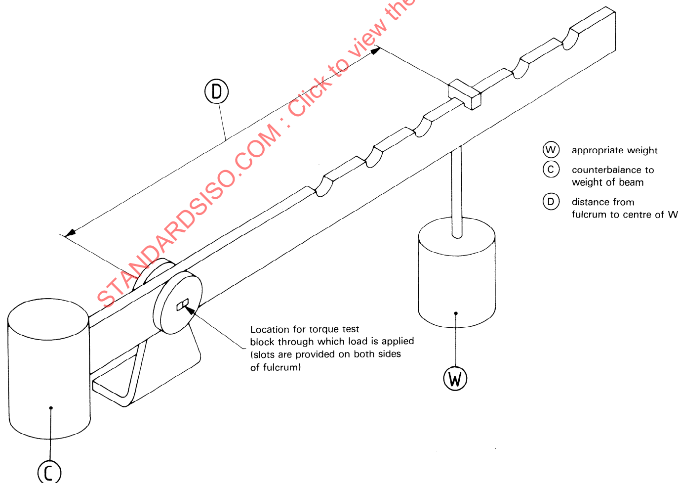
Figure 5 — Diagrammatic representation of the principle of a torque-testing device
