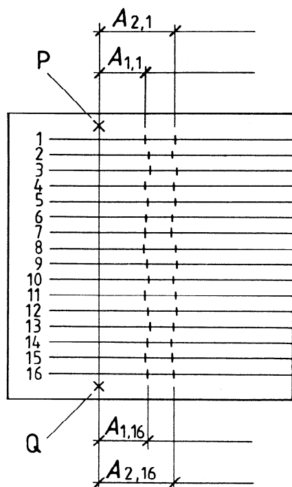
Figure 6 — Masking sheet on target card
