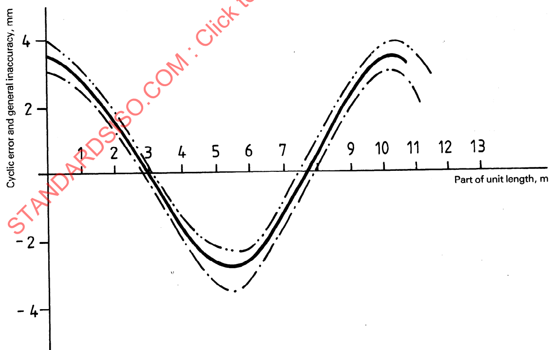
Figure A.3 — Mean of the lines shown in figure A.2
