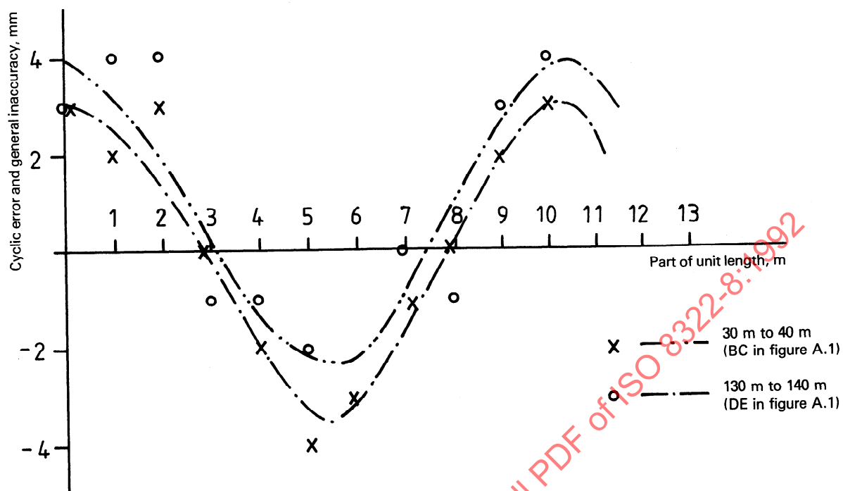
Figure A.2 — Graphical representation of cyclic error
