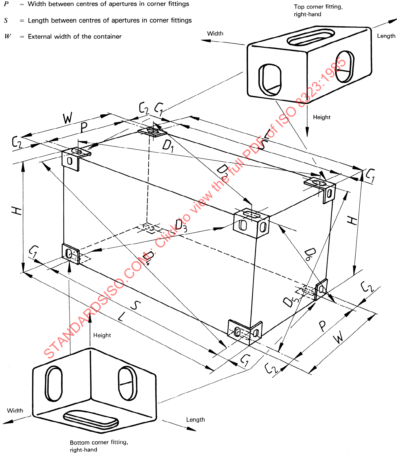
Figure 13 — Corner fittings
