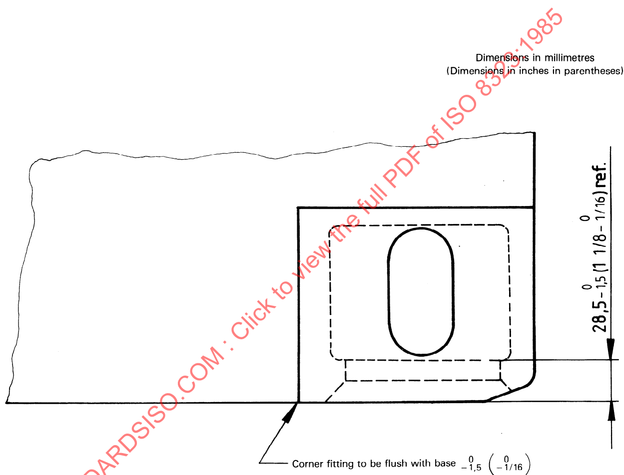
Figure 9 — Location of bottom corner fitting
