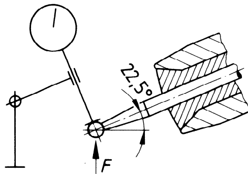
Figure 5 — Test piece at 22,5^\circ to horizontal
