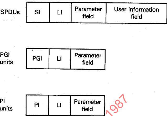
Figure 5 — Illustration of structure of SPDUs, PGI and PI units
