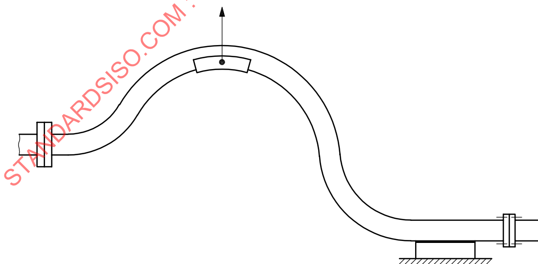
Figure 1 — Supports for hose during temporary installation
