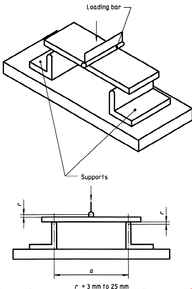
Figure 3 — Bending test machine layout
