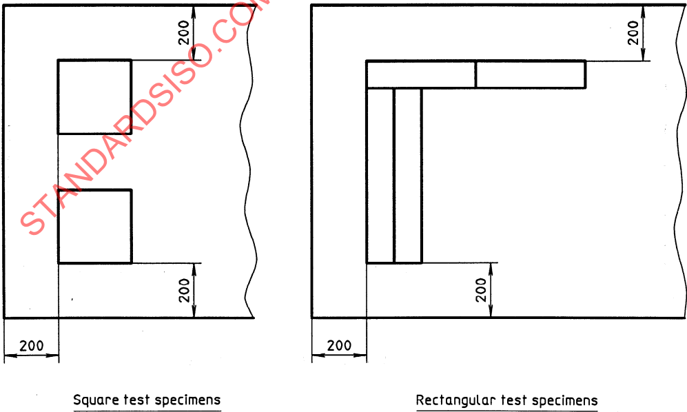
Figure 2 — Cutting of test specimens
