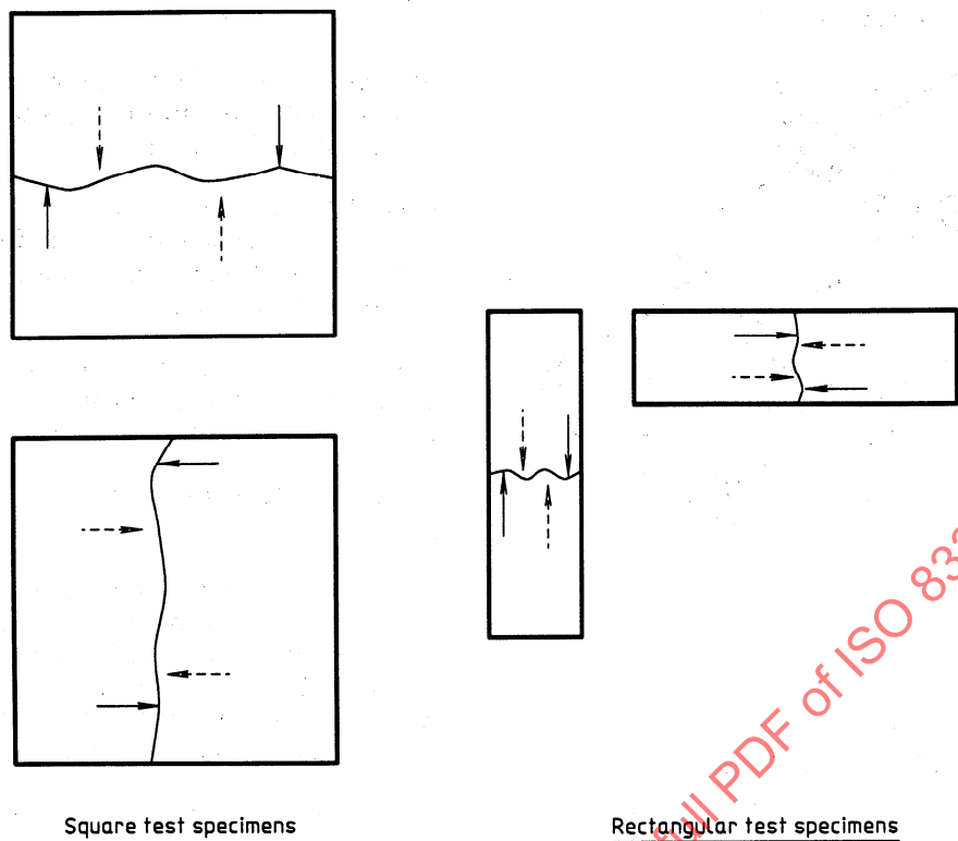
Figure 4 — Measurement of thickness of specimens
