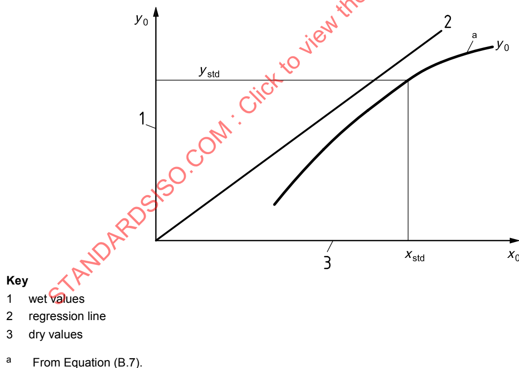
Figure B.1 — Regression line for wet/dry values with lower confidence level
