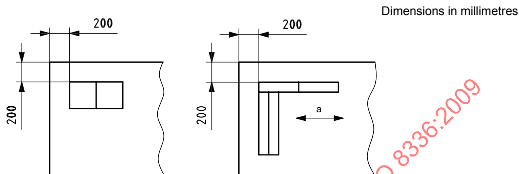
Figure 1 — Adjacent specimen cutting
