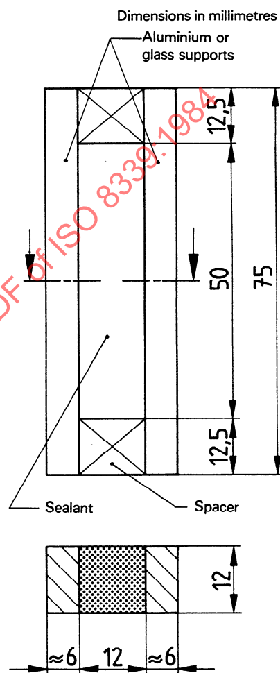
Figure 2 — Test specimen with aluminium or glass supports
