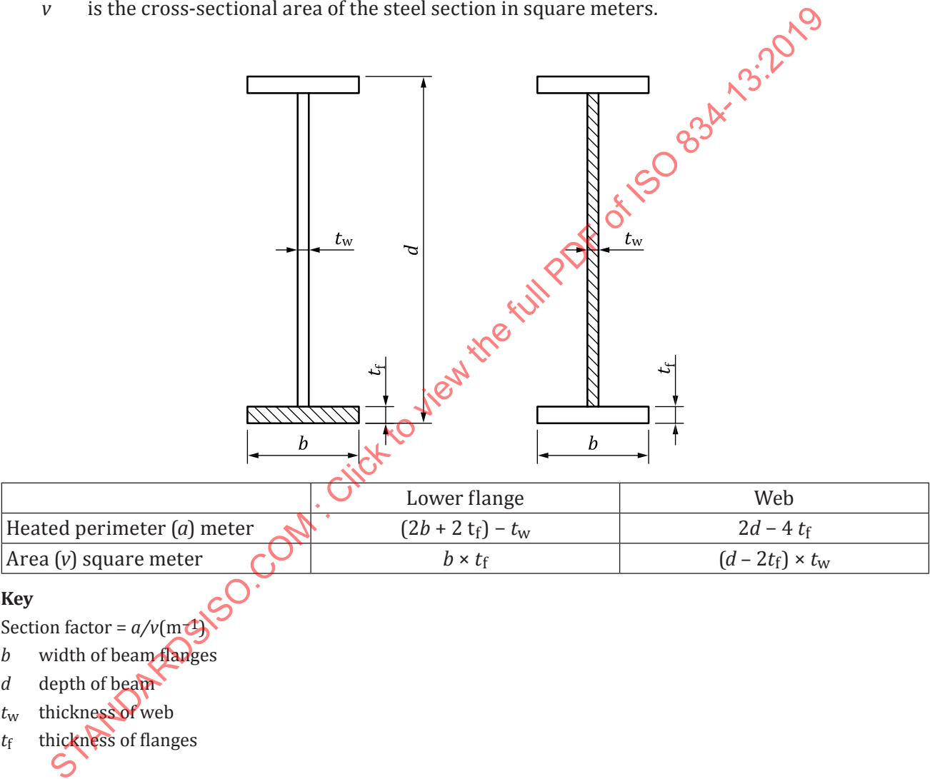
Figure 7 — Elemental section factor
