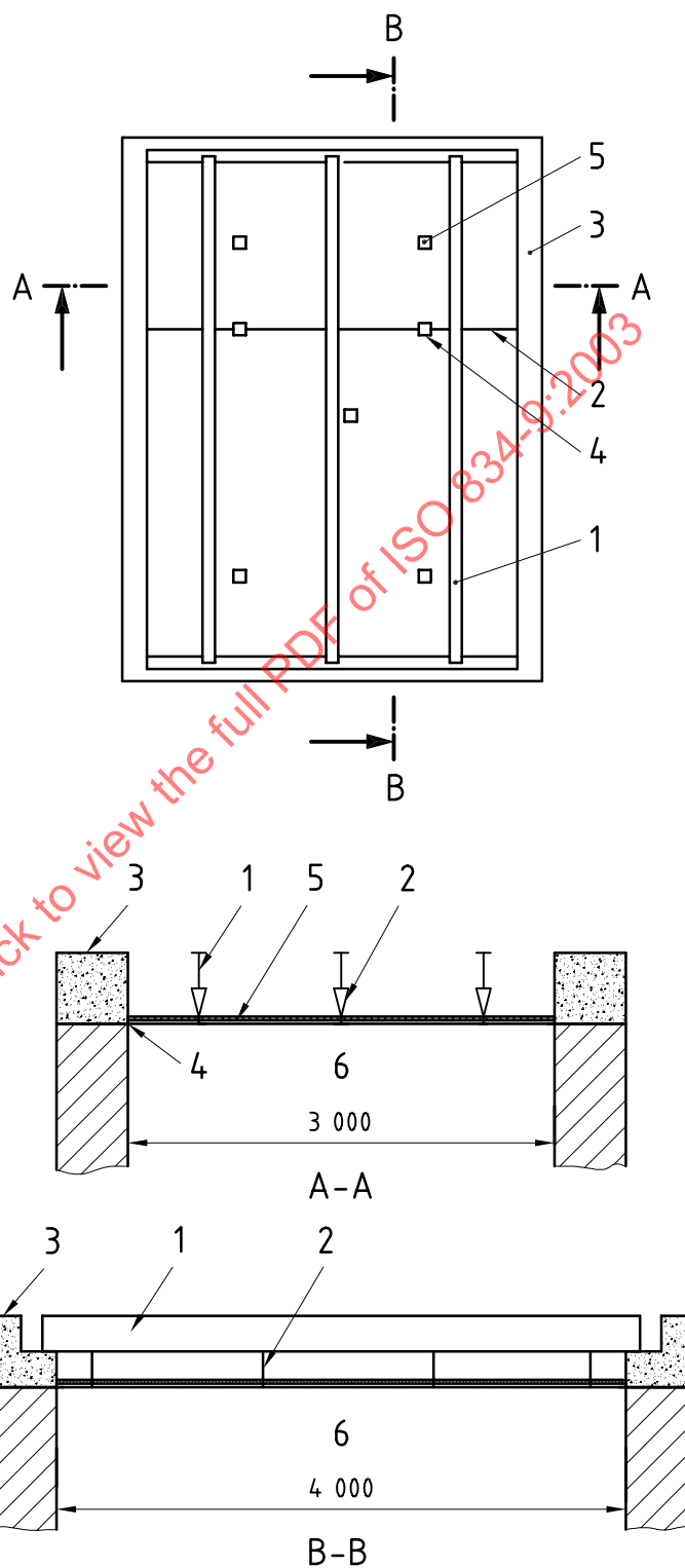
Figure 1 — Ceiling exposed to fire from below — Suspended (shown) or self-supporting
