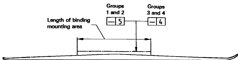
Figure 2 — Longitudinal profile of the surface
